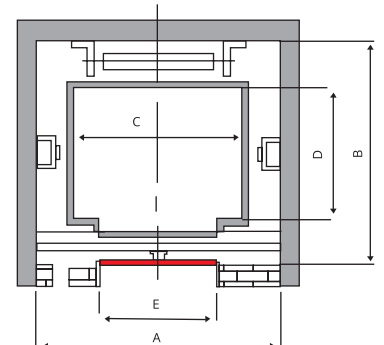
HOISTWAY MACHINE ROOM PLAN FOR AUTO DOOR
